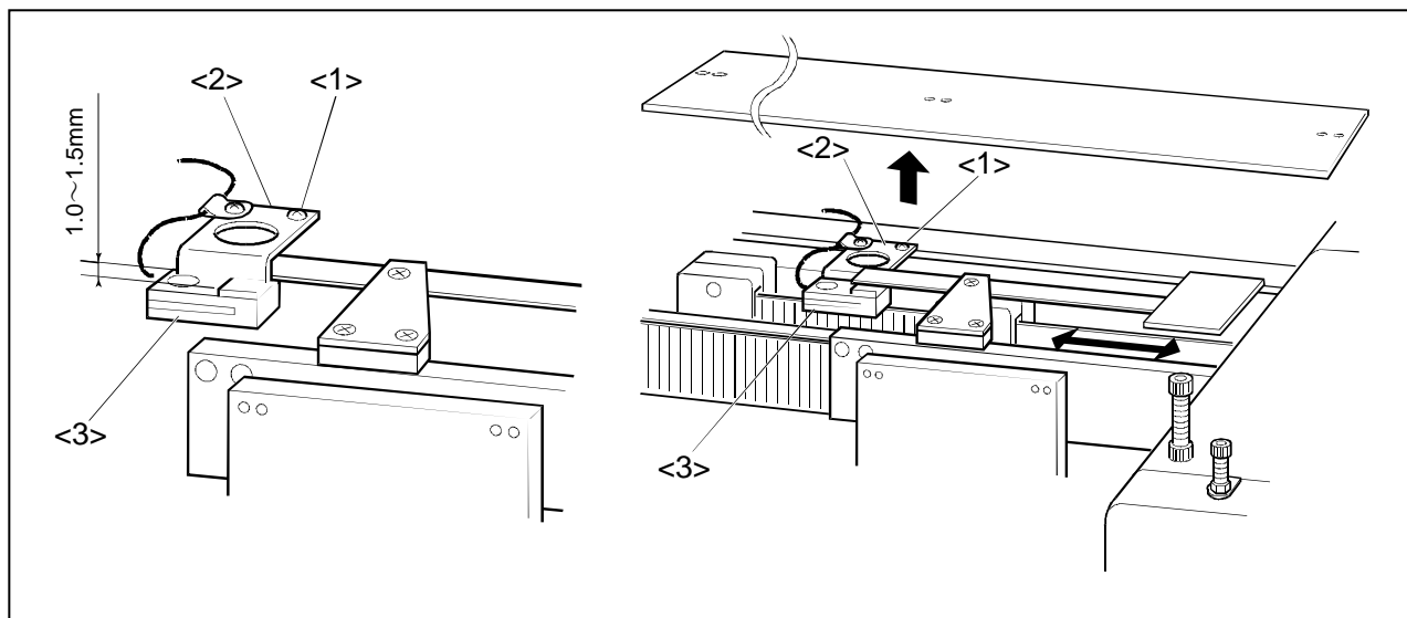
<1>: Set screw <2>: Detector set plate <3>: X detector
