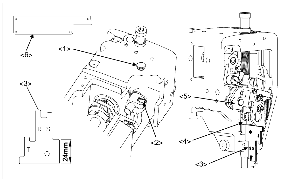
<1>: Rubber plug <2>: Arm set screw <3>: Gauge <4>: Presser bar holder <5>: Presser foot lifting lever <6>: PF motor cover
