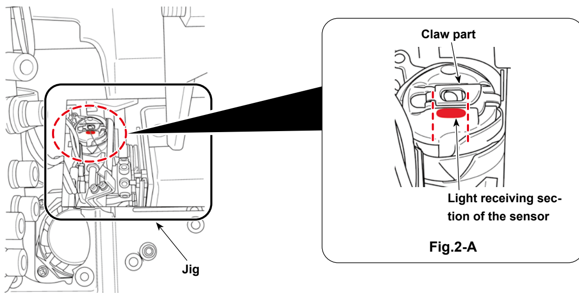
Fig.2 Sensor light irradiation position
