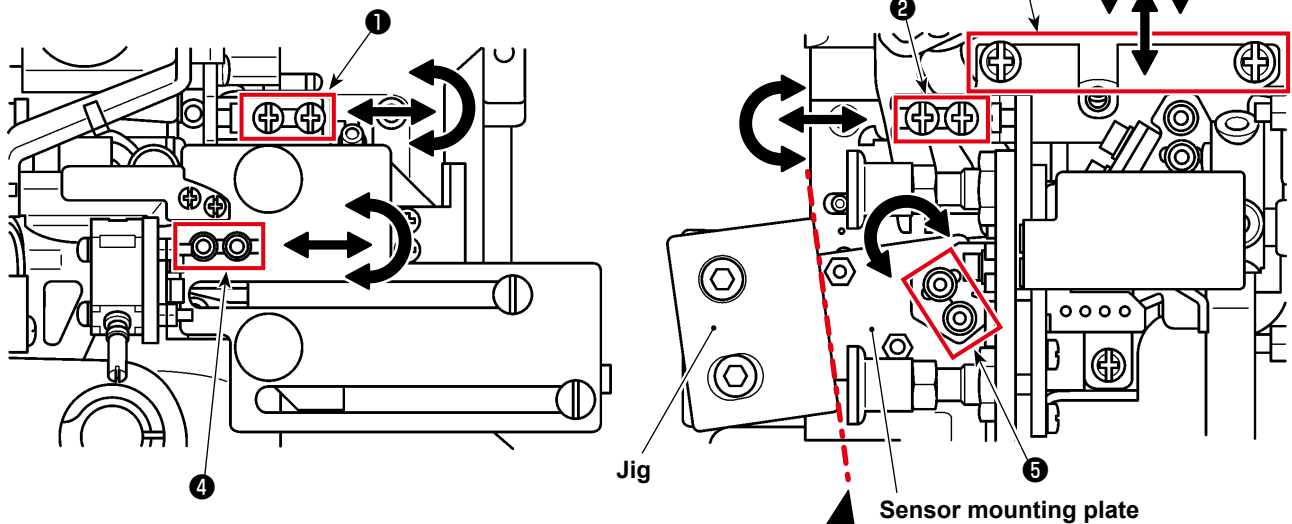
Fig.1 Sensor position adjustment points
