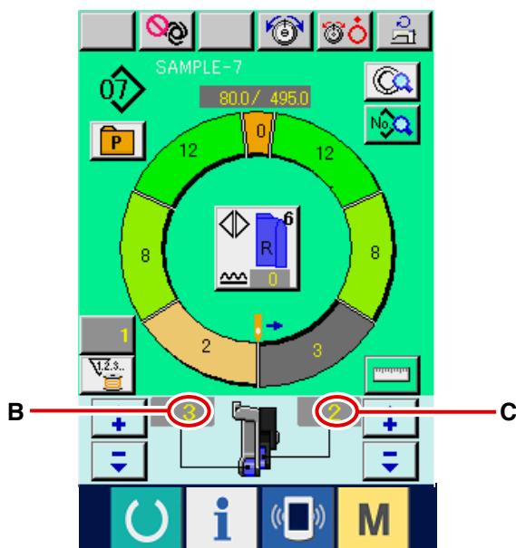
Sewing screen
