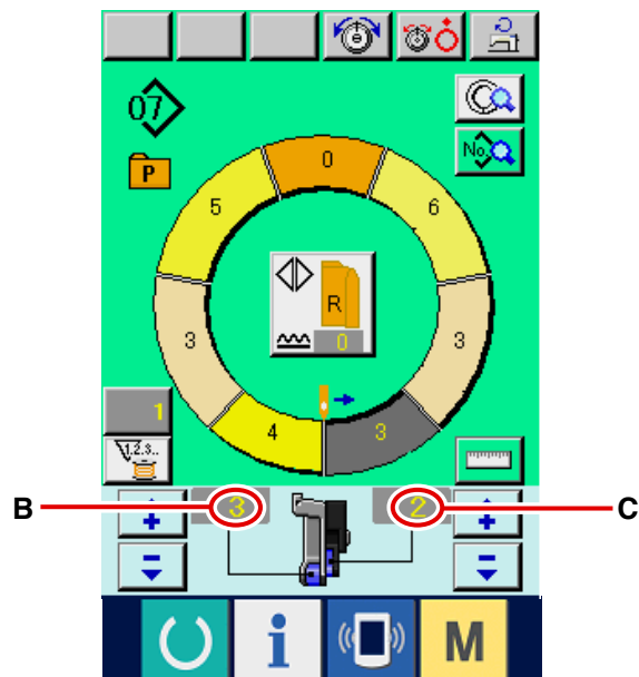
Sewing screen
