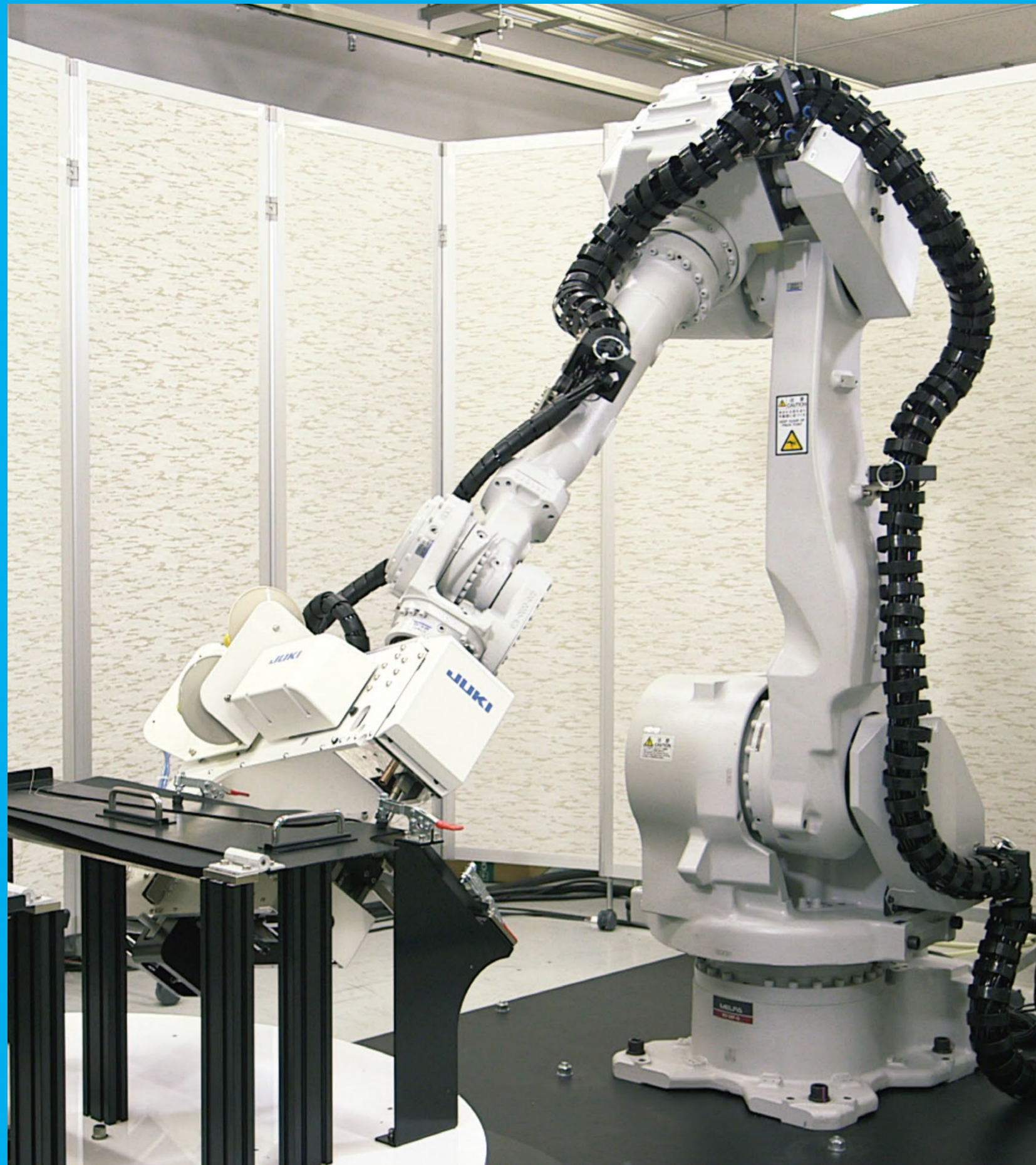
Robot Sewing System
