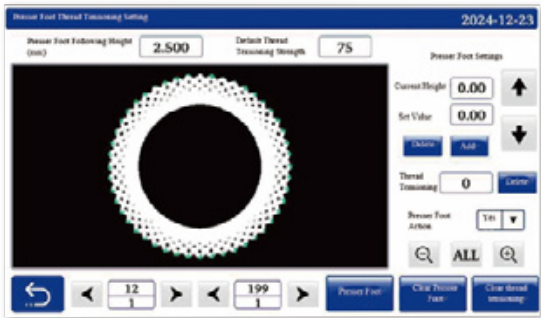
Program screen
